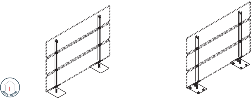
Struttura freestanding per 3 pannelli privacy orizzontali Freestanding support for 3 privacy horizontal panels
